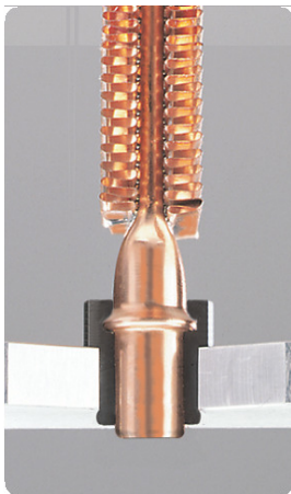
M-core Radiator
